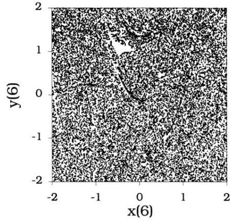
FIG. 2. The basin (black dots) of the chaotic attractor with \lambda_1 \approx 0.18 in Fig. 1. Blank regions denote basins of the quasi-periodic and periodic attractors.
